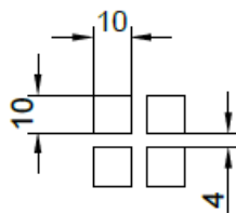
Square perforation
