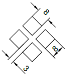
Rhombus perforation
