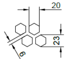
Honeycomb perforation
