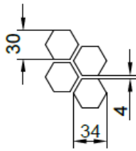
Honeycomb perforation
